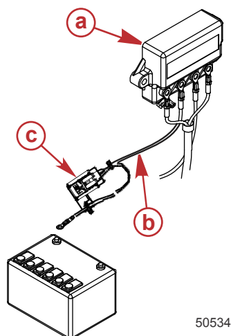
a - MerCathode b - Fil rouge/violet c - Fusible de 5 A
