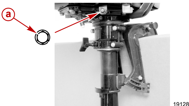
a - Drain plug
