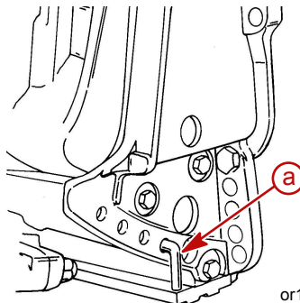
a - Stainless steel tilt pin (Three-Ram trim system)
