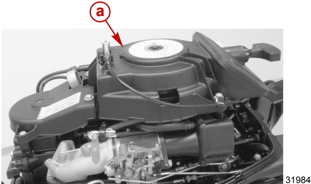
a - Handstarter
